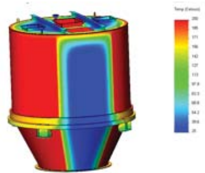
Figure 7 Temperature distribution
